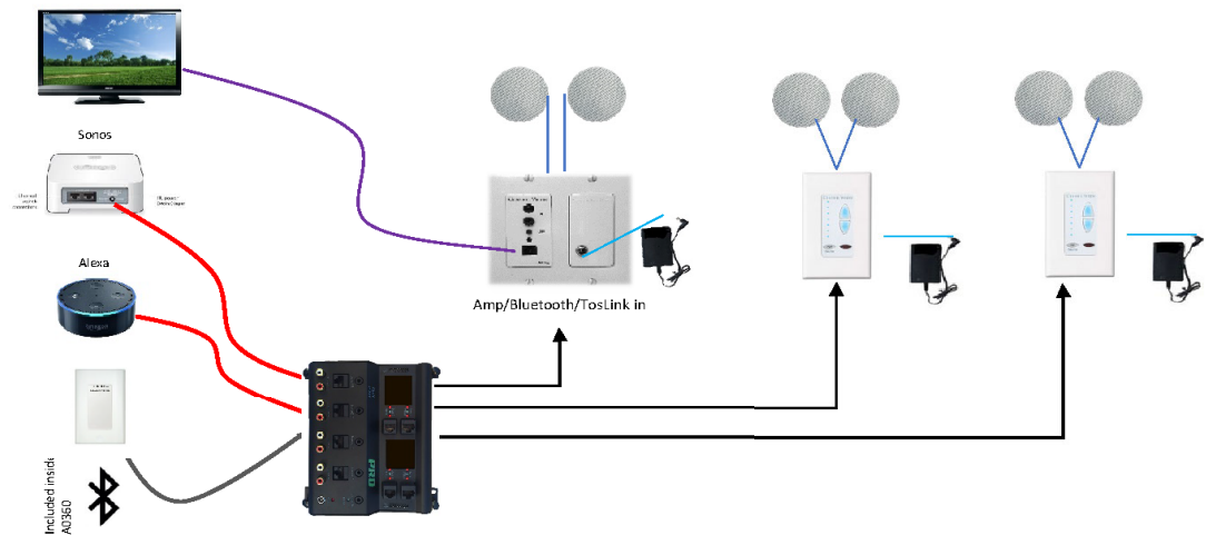
Multi-Room System
